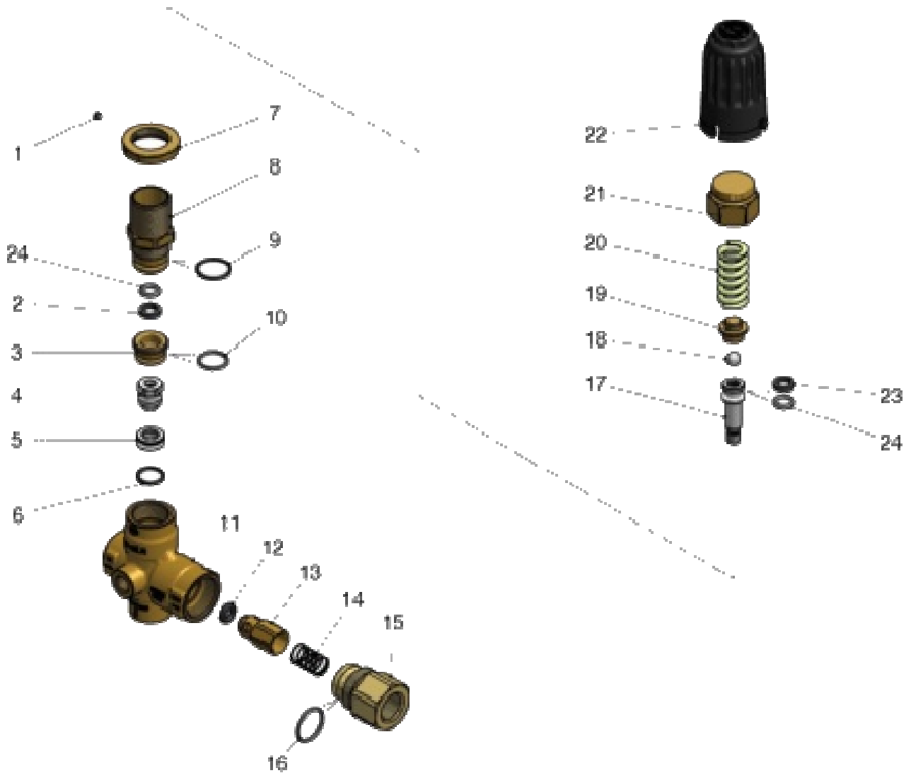
SPARE PARTS KIT
