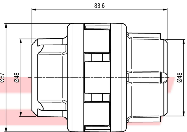
New Flexible Couplings NMT Series
